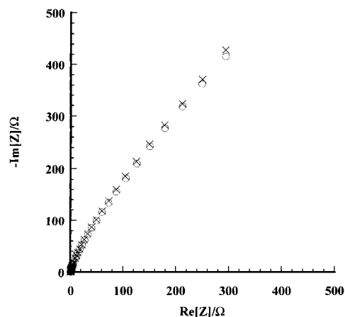
Fig. 5. Exemplary plot of Kramers–Kronig transform (×) of the measured (○) impedance spectra. Diagram recorded at gold electrode in (63–27–10) mol % (Li–Na–K)CO 3 , T = 923 K.
