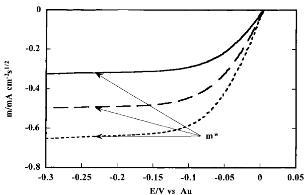
Fig. 3. Semiintegral curves corresponding to voltammograms presented in Figure 2. P_{total} : (—) 1, (---) 3 and (- - -) 5 atm.
