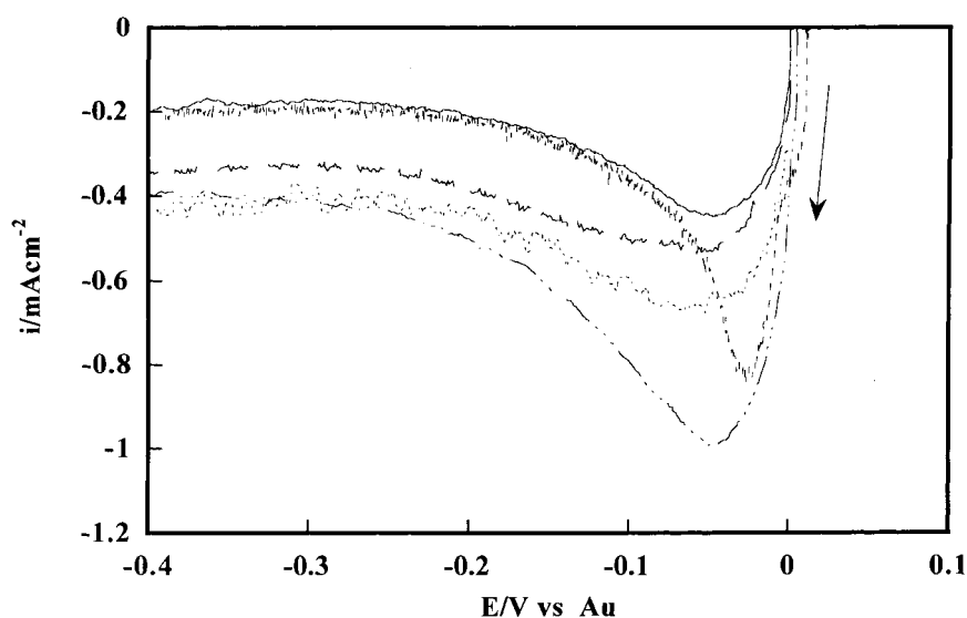
Fig. 1. Effect of melt composition on voltammograms run at gold flag electrode under 1 atm of \text{O}_2/\text{CO}_2 = 90/10 at 923 K. Scan rate 1 \text{ V s}^{-1} . (Li–Na–K) \text{CO}_3 : (– – –) 53–47–0; (—) 62–0–38; (—) 63–27–10; (· · · · ·) 48–12–40 and (— · · · ·) 26.7–23.3–50.
